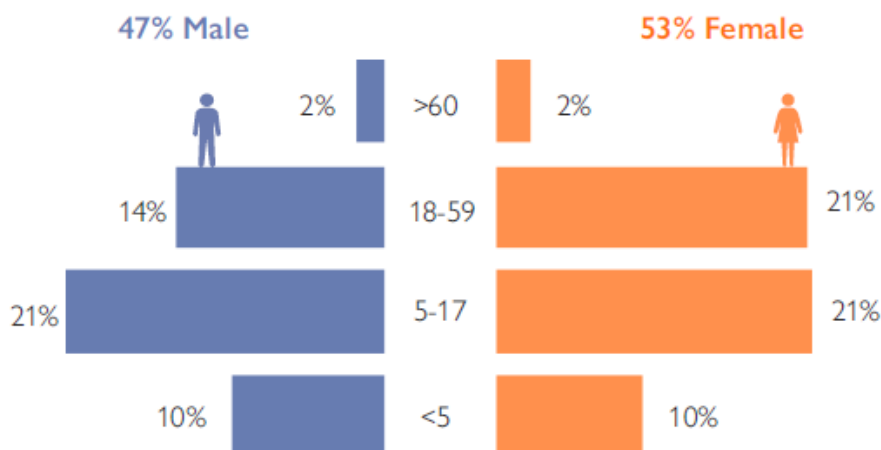
Population pyramid (n=74,888 individuals)
